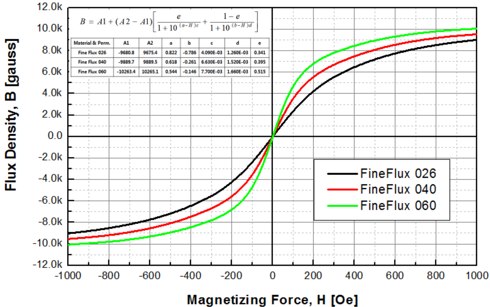
Fine Flux Core BH Curve
